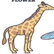
GIRAFFE
